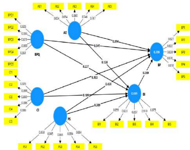
Figure 1: Outer Measurement Model
