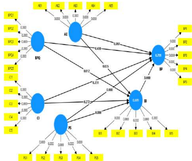
Figure 2: Inner Structural Model
